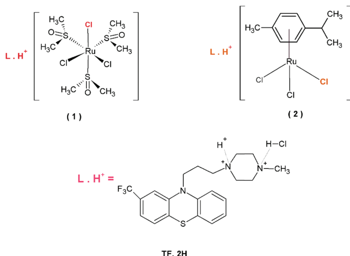
Scheme 1. General formulae of complexes: (TF.2H)[Ru(DMSO) 3 Cl 2 ]Cl·0.5C 2 H 5 OH ( 1 ) and (TF.2H)[RuCl 2 (η 6 - p -cymene)]Cl·0.5C 3 H 7 OH·0.5H 2 O ( 2 ), where TF.2H is protonated trifluoperazine
