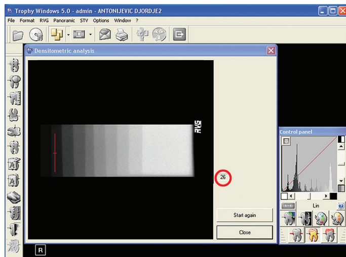
Figure 2. Radiographic image of the aluminum step wedge obtained by Trophy for windows digital radiographic system. Red line indicates the place of the gray scale value measurement (2 mm thickness). The value of the grey scale is encircled in red.
